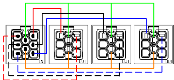
8-Wire 3L, 3N, 2G Phase Selector
