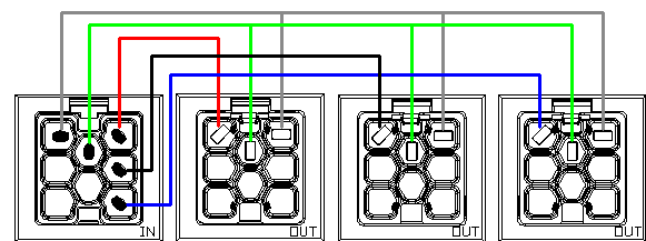
5-Wire 3-Phase Selector (347/600V 20A shown)
