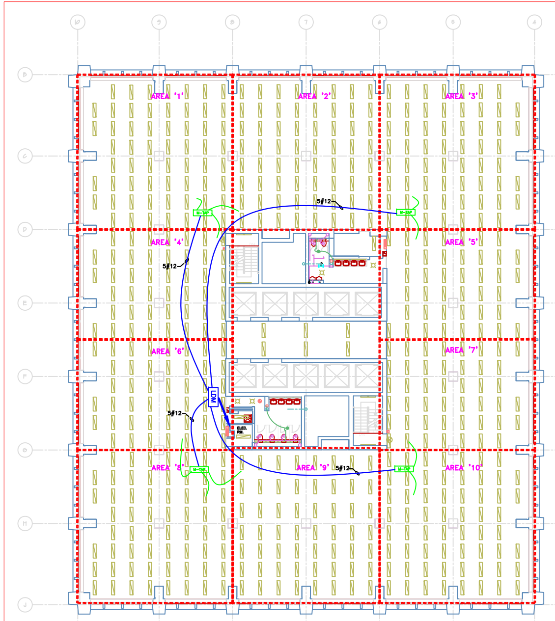
1 347V LIGHTING LAYOUT SCALE 1 : 100
